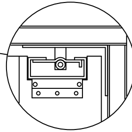
GS-HINGE ASSEMBLY
